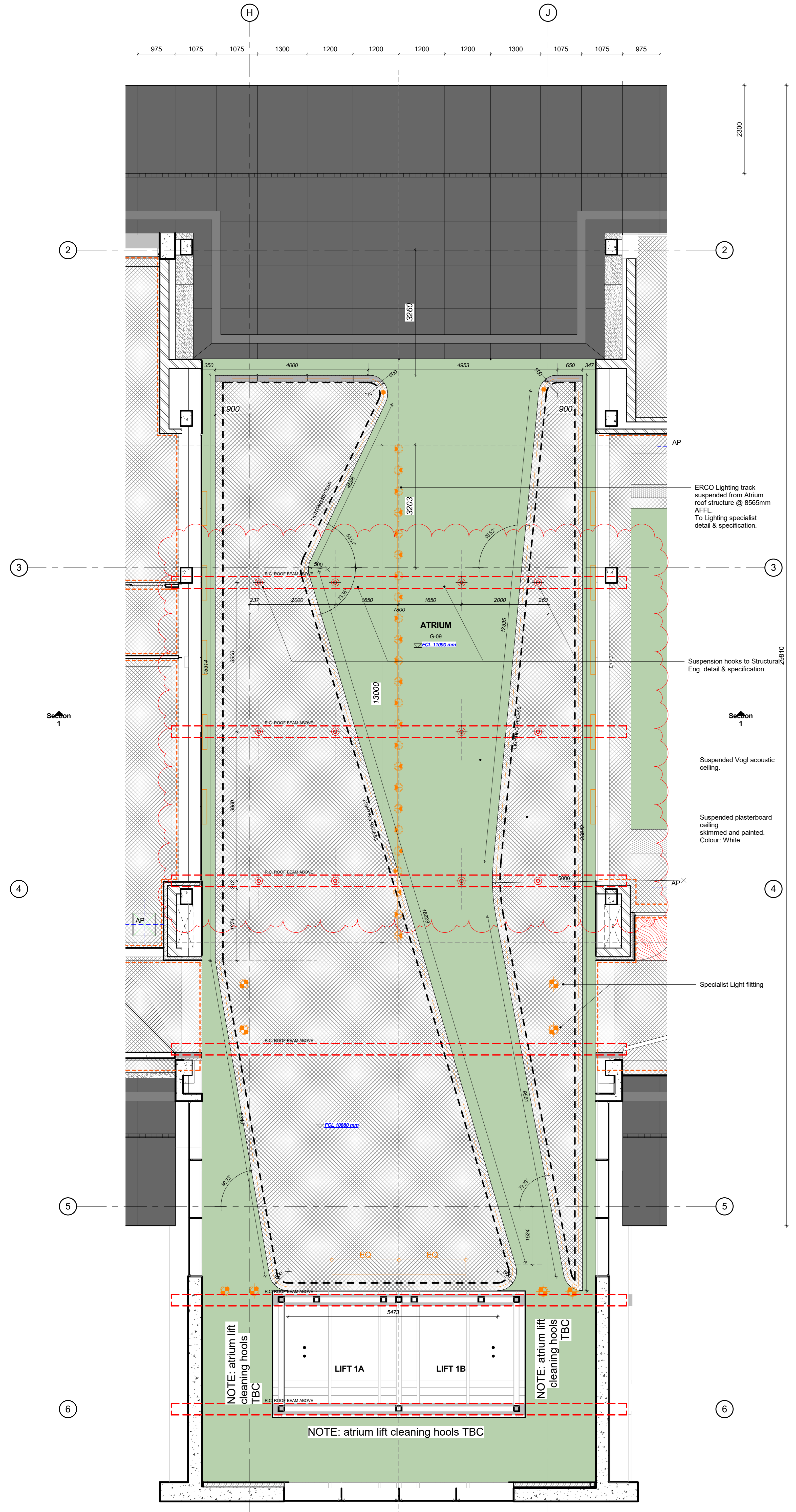
FIRST FLOOR: Atrium Ceiling Plan SCALE 1:50
