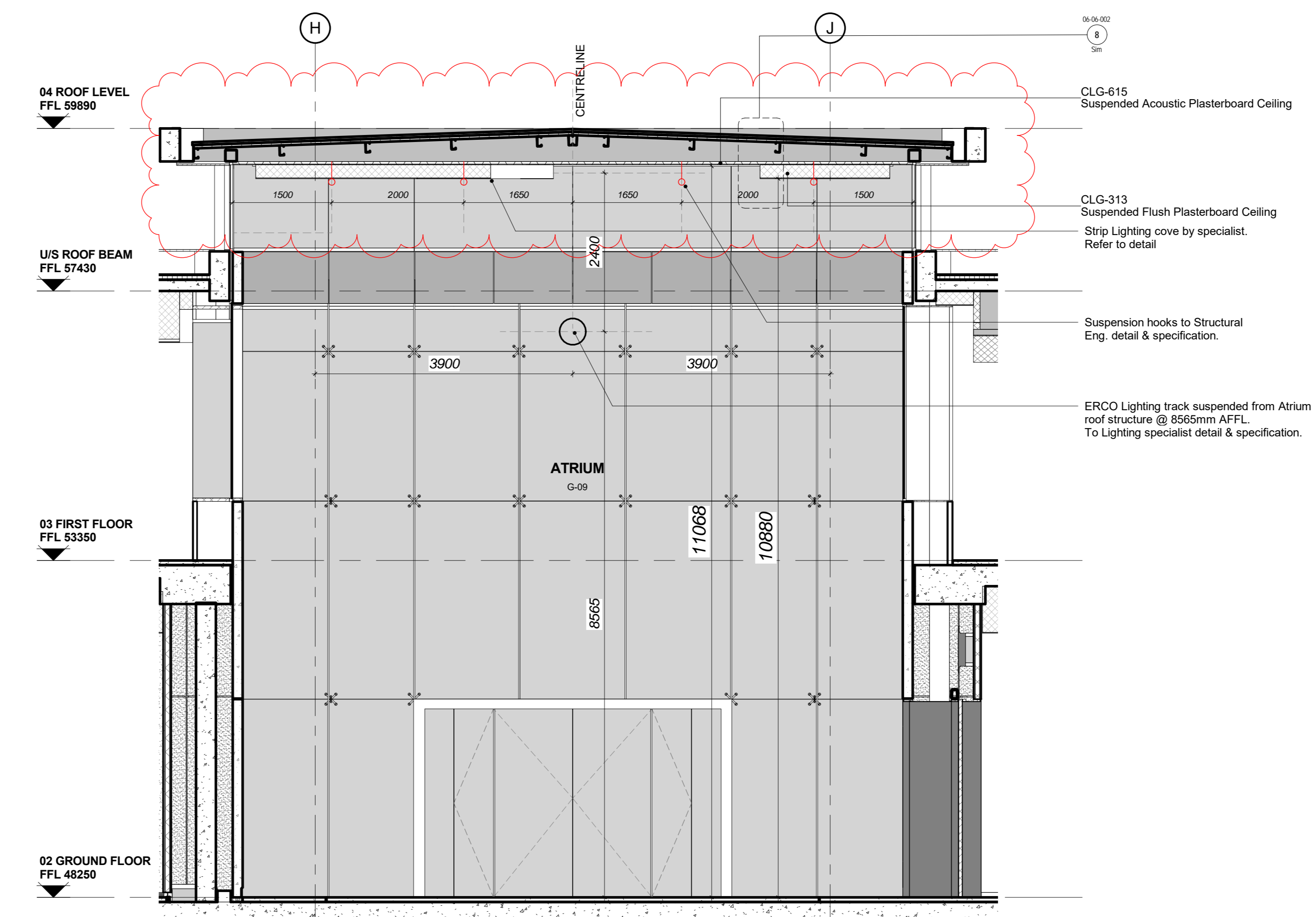
Atrium Ceiling Section 1 SCALE 1:50
